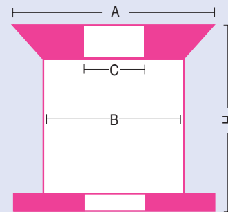
Spule DL100 spool DL100
